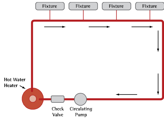
Figure 3. Demand-Initiated Hot Water Recirculating System
