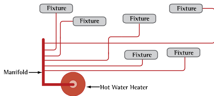
Figure 4. Whole House Manifold System
