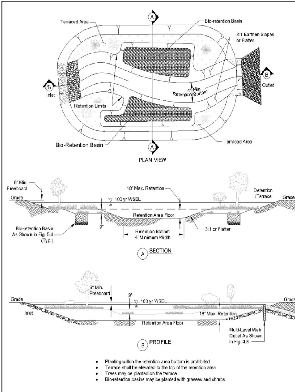
Figure 5.5 Terraced Detention Basin with Retention
