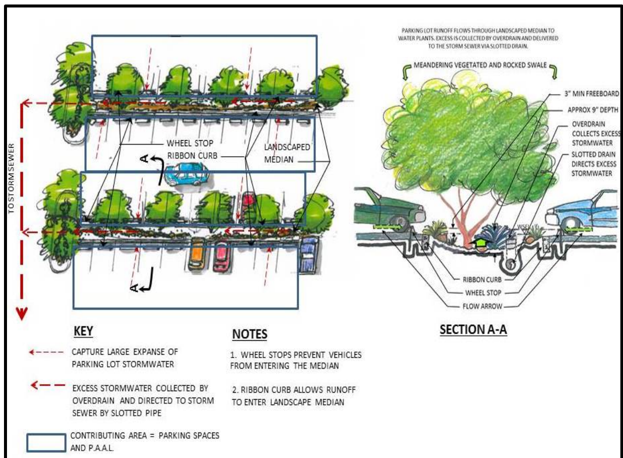
Figure 2.4 Parking Lot with Stormwater Runoff Directed to Basins Elevated Grate Inlet Maximizes Stormwater Harvesting
