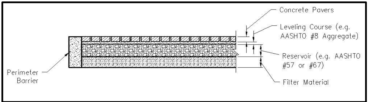
Figure 5.8 PICP Cross Section
