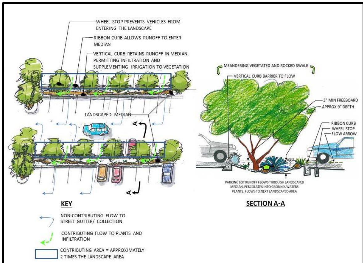
Figure 5.3 Expanded Area Non-contributing Basin in a Parking Lot Median
