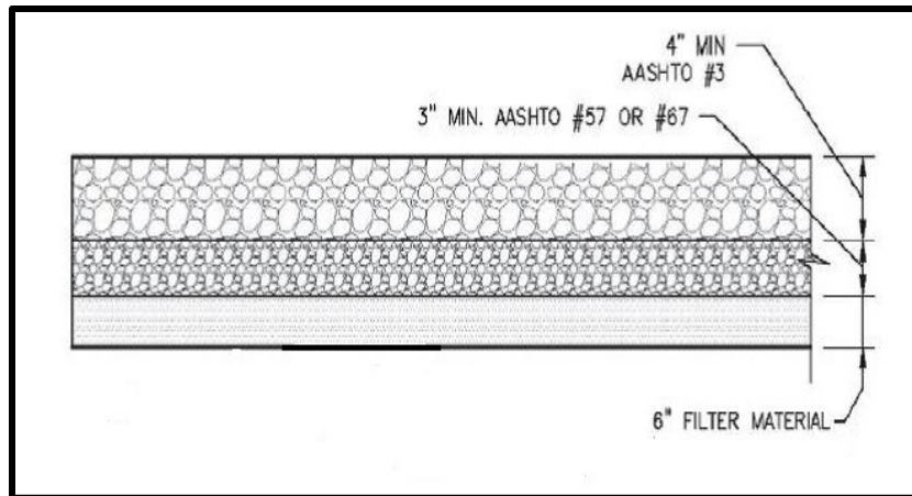
Figure 5.6 Porous Gravel Cross Section
