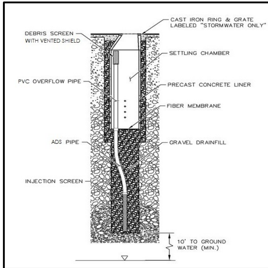
Figure 4.8 Typical Dry Well Installation
