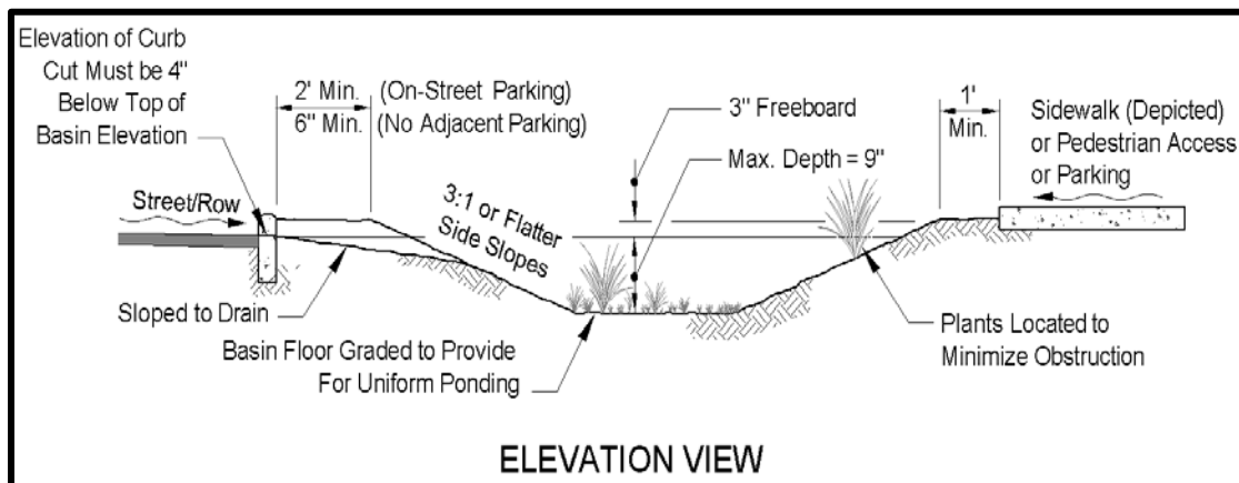
Figure 5.2 Roadside Stormwater Harvesting Basin
