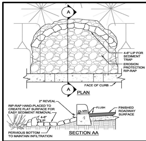
Figure 5.1 Sediment Trap
