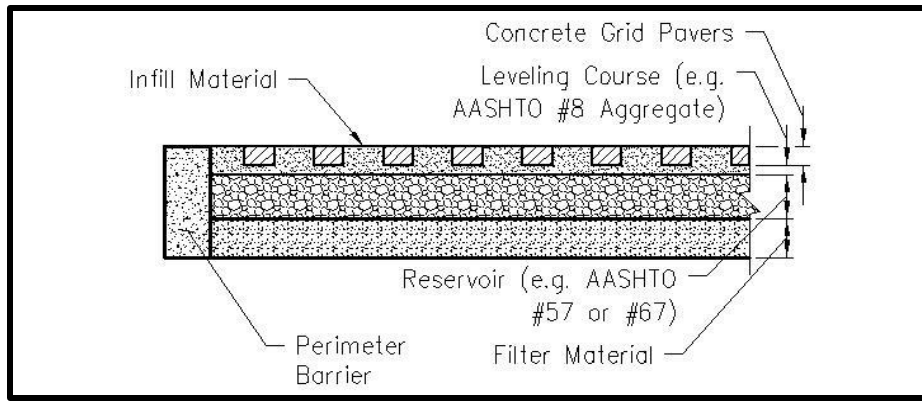
Figure 5.7 Concrete Grid Cross Section
