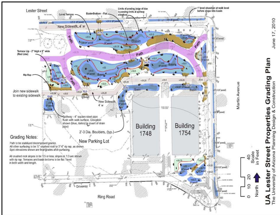
Figure 1.1 An Example LID Site Design (University of Arizona, Department of Planning, Design & Construction).
