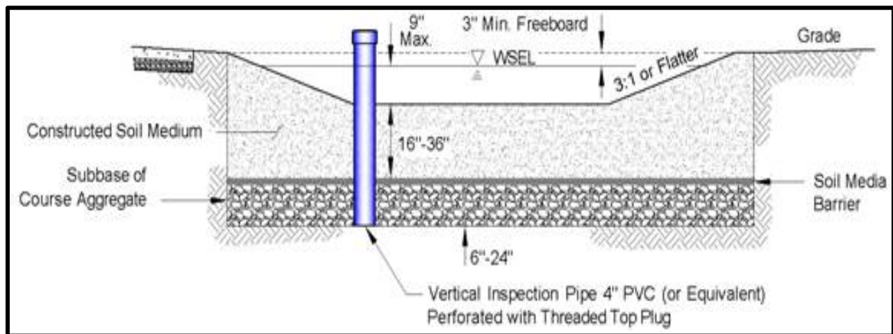
Figure 5.4 Bioretention Basin
