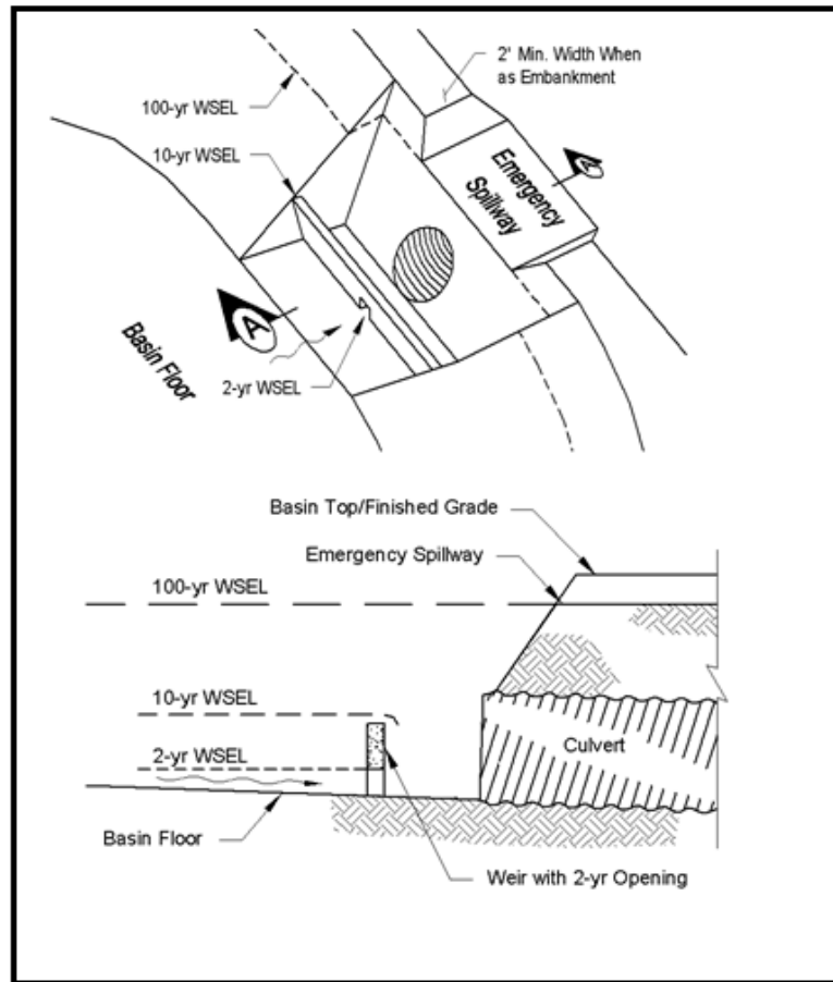
Figure 4.6 Combination Weir – Culvert Outlet
