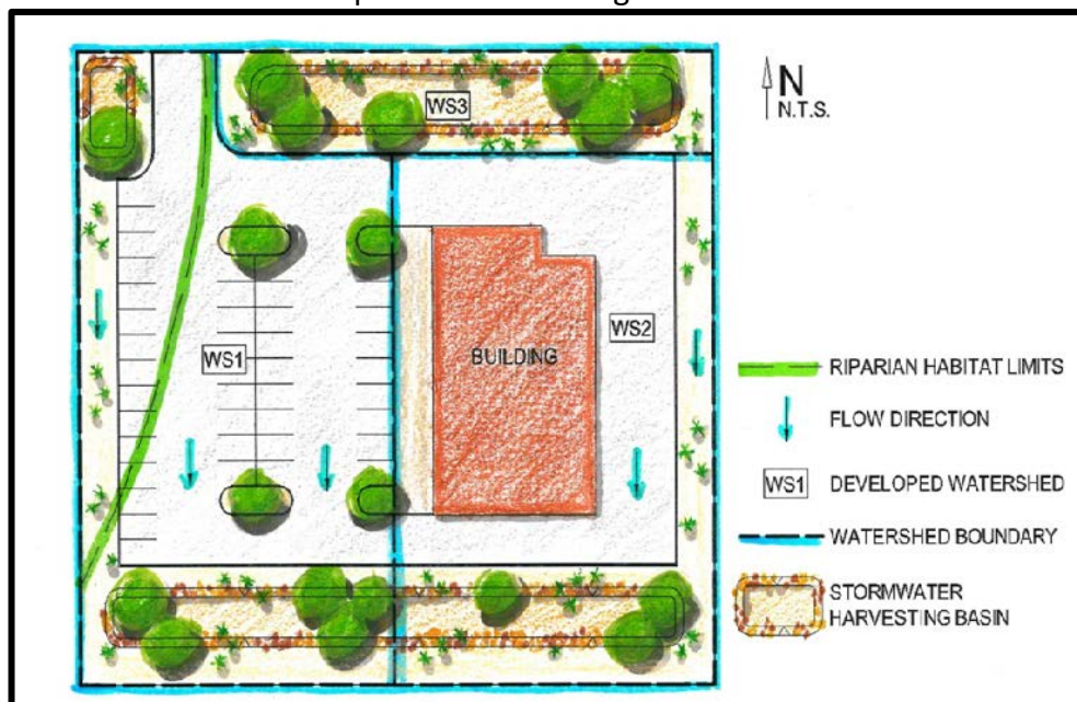
Figure 2.1 First-flush Example Developed Watersheds
