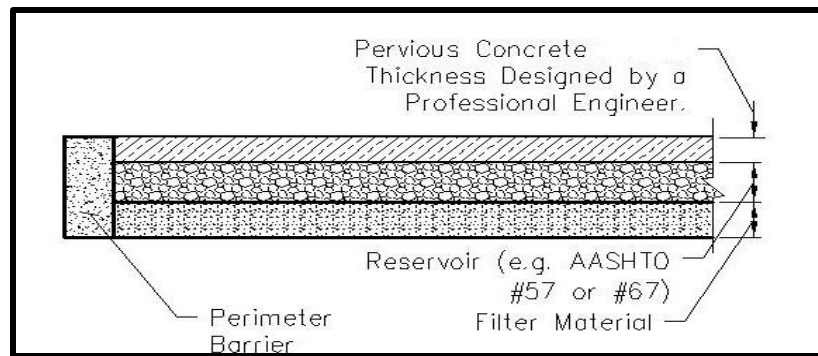
Figure 5.9 Pervious Concrete Cross Section
