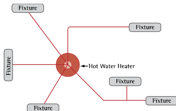
Figure 2. Core Plumbing System
