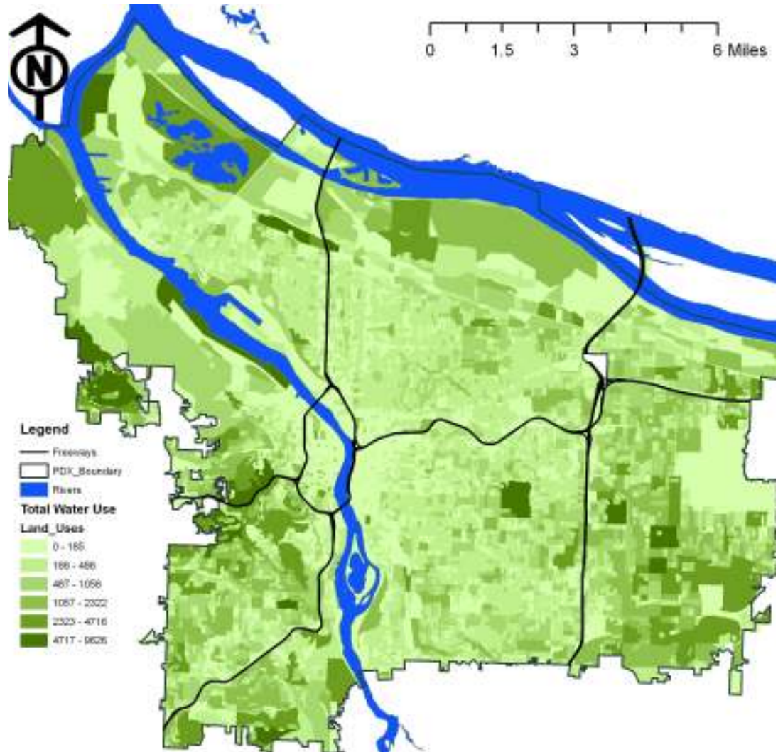
Figure 1: Total daily water use (gallons) among of all land uses in Portland Oregon (Census Block geography).
