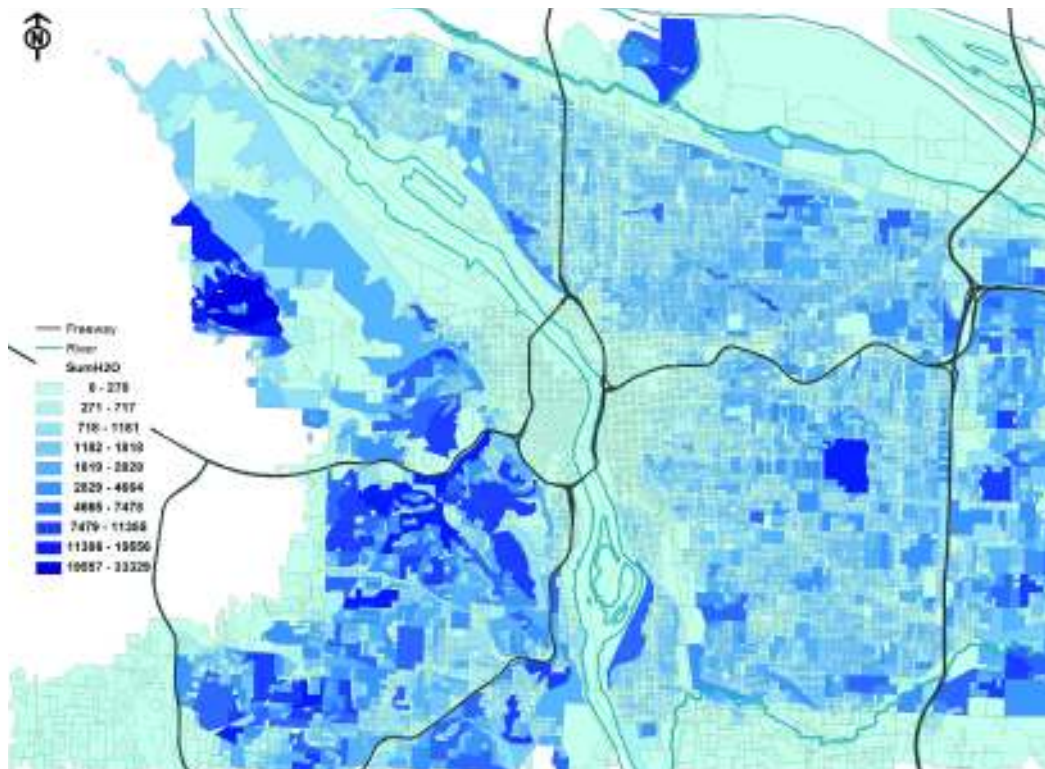
Figure 2: Total daily water use (gallons) among SFR households in Portland Oregon (Census Block geography).
